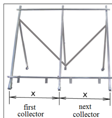
Version with struts (additional option)
