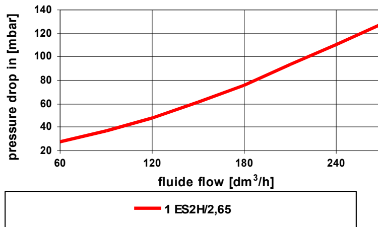
Pressure loss by flow through 1 meander panels ES2H/2,65
